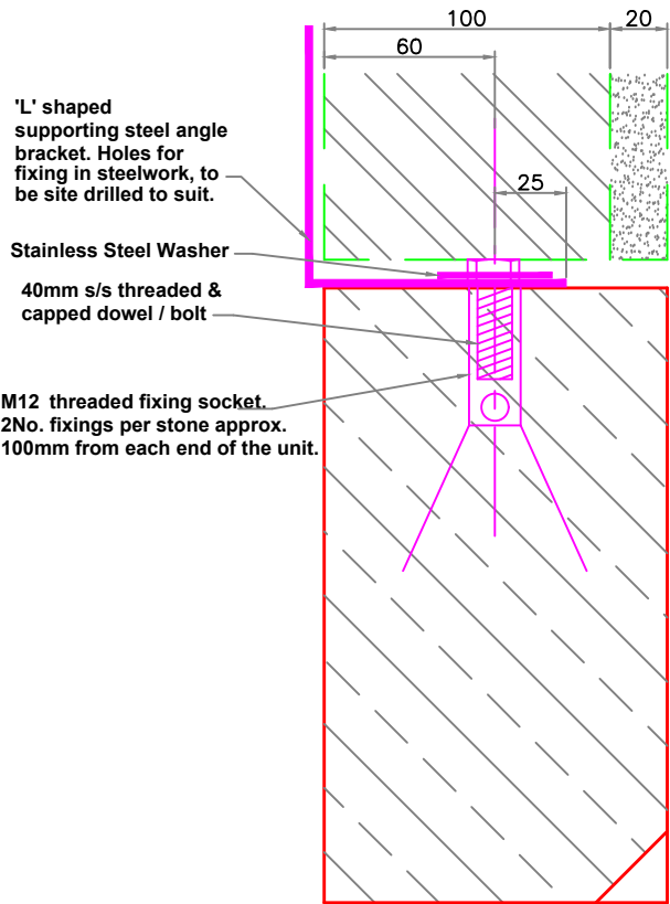
Top Hanging Restraint Detail
