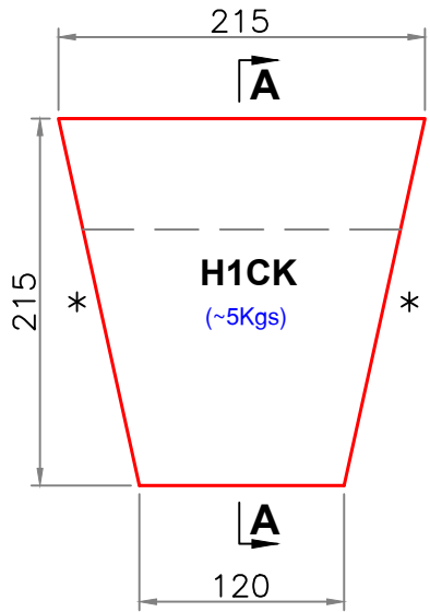
H1CK - Elevation
